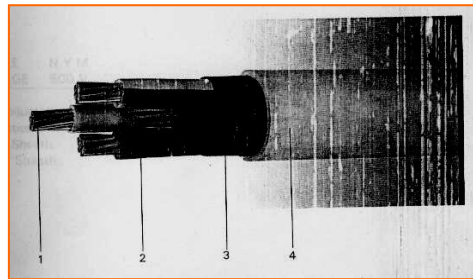
Gambar 3 Kabel NYM
