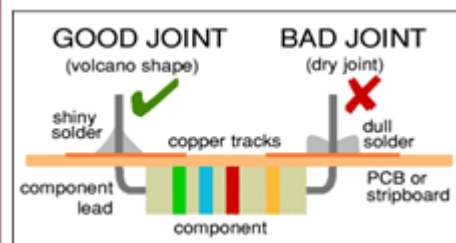
Gambar 42 Hasil solderan
