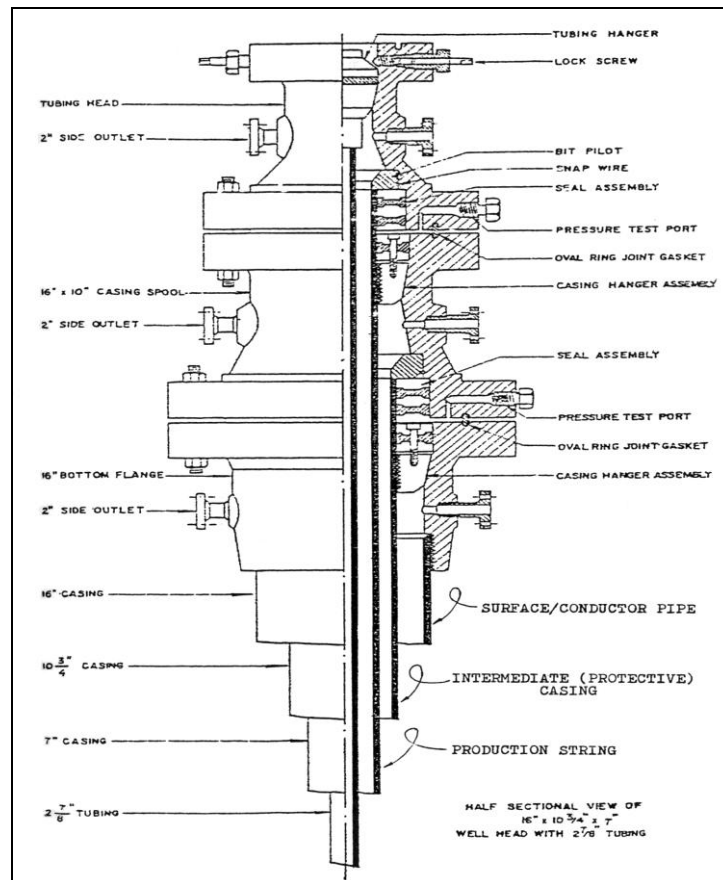
Gambar 8.11. Wellhead dan Safety Valve
