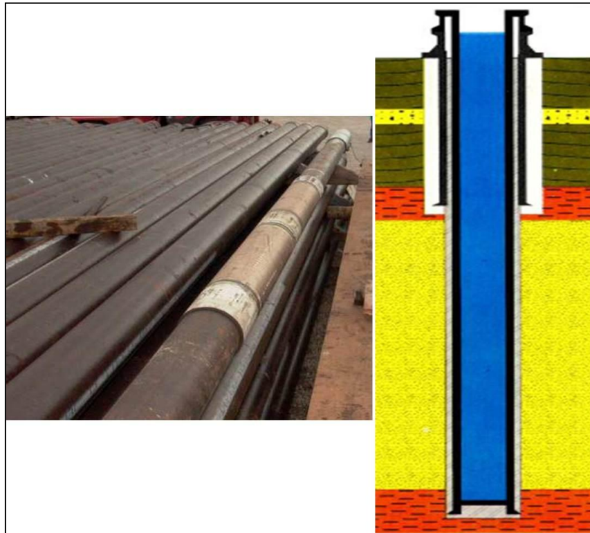
Gambar 5.3. Surface Casing
