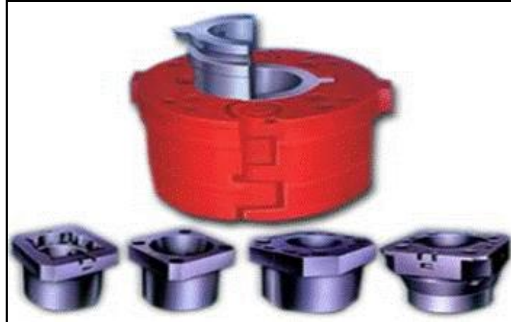
Gambar 4.16. Master Bushing tipe split
