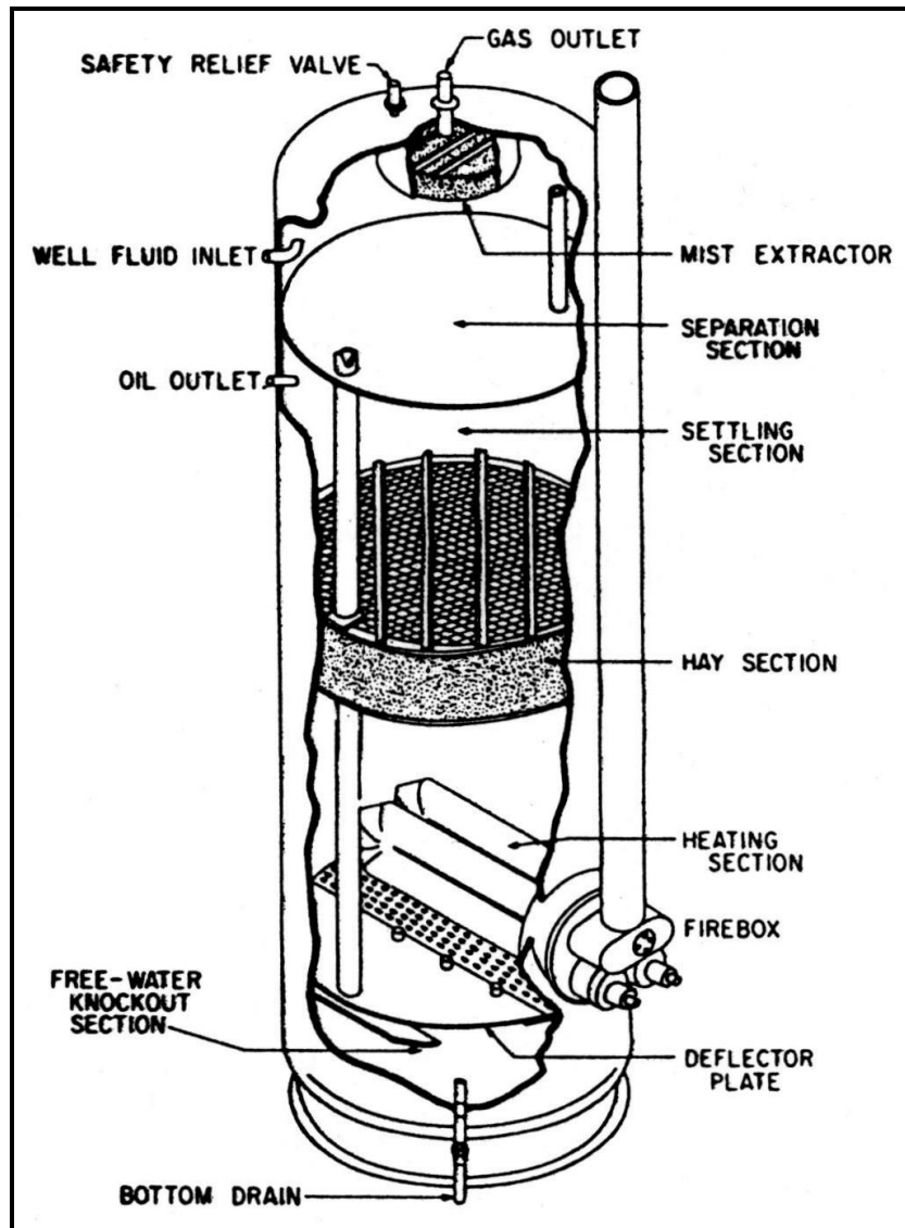
Gambar 8.21. Vertical Treater
