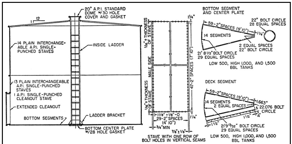
Gambar 8.23. Penampang Storage Tank Jenis Bolted-Steel Tank
