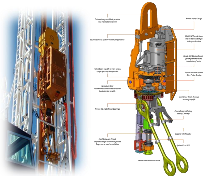
Gambar 4.23. Top Drive
