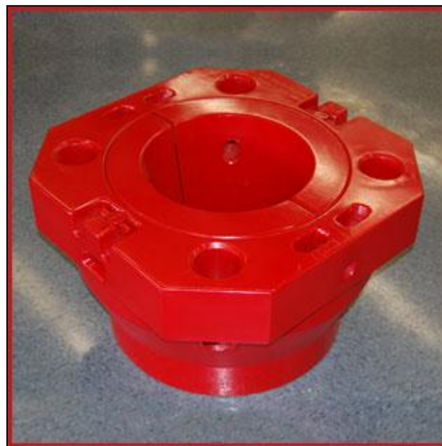
Gambar 4.15. Master Bushing tipe solid
