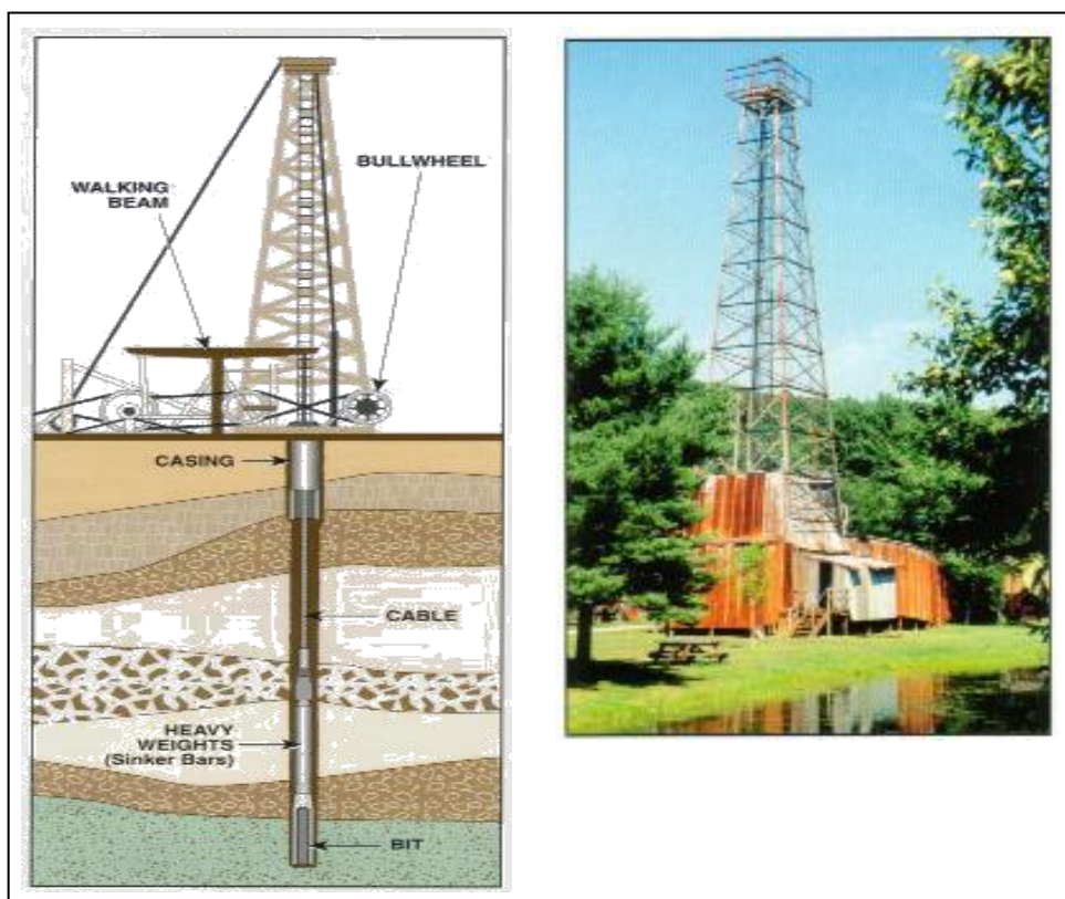
Gambar 1.1. Skema Cable Tool Drilling .
