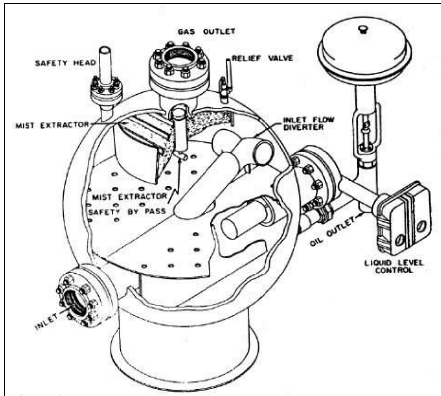
Gambar 8.19. Separator Spherical Tekanan Rendah
