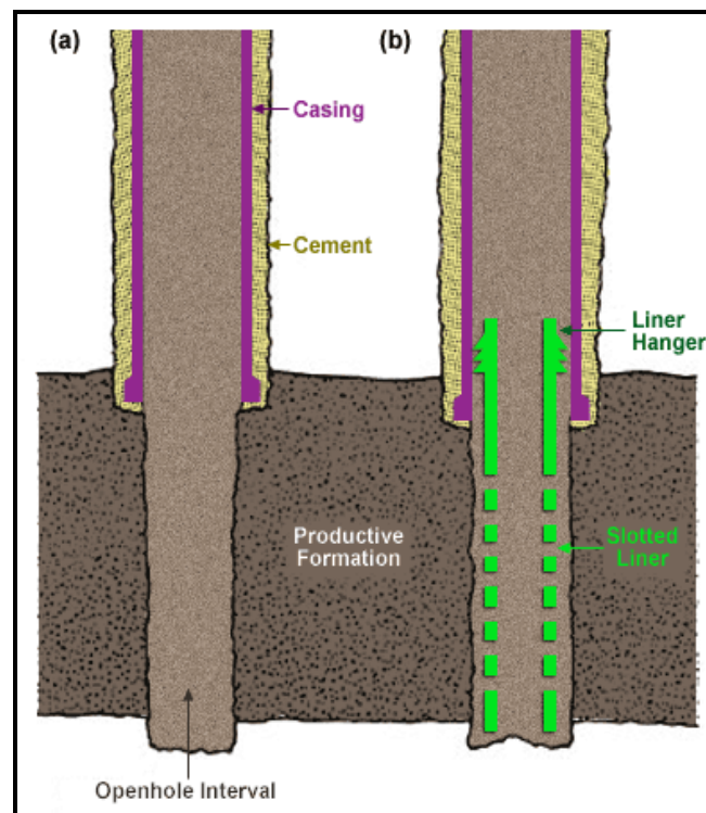
Gambar 6.1. Open Hole Completion
