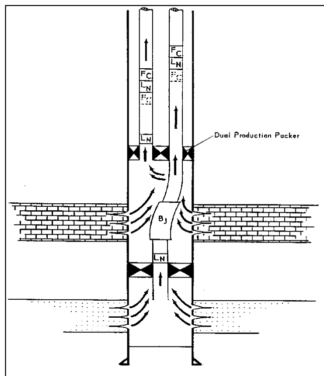
Gambar 6.3. Multiple Completion
