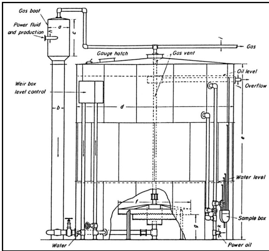
Gambar 8.20. Wash Tank
