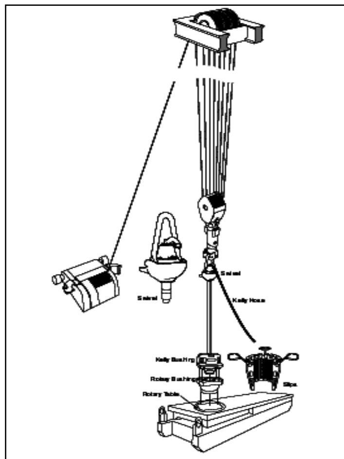
Gambar 4.10. Sistem Putar ( rotating system )
