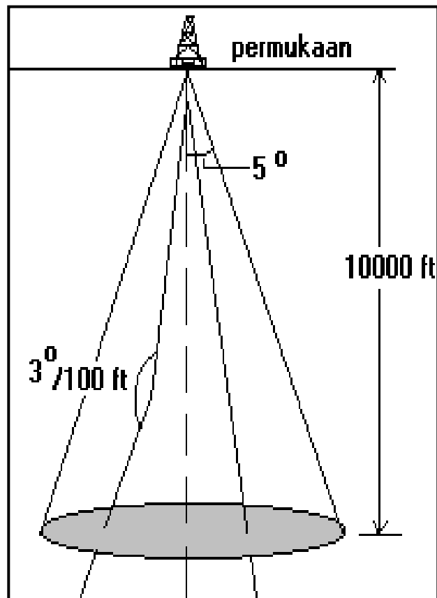
Gambar 3.6. Straight Hole Drilling
