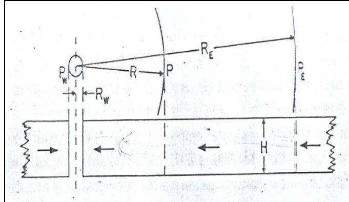
Gambar 8.3. Aliran Radial
