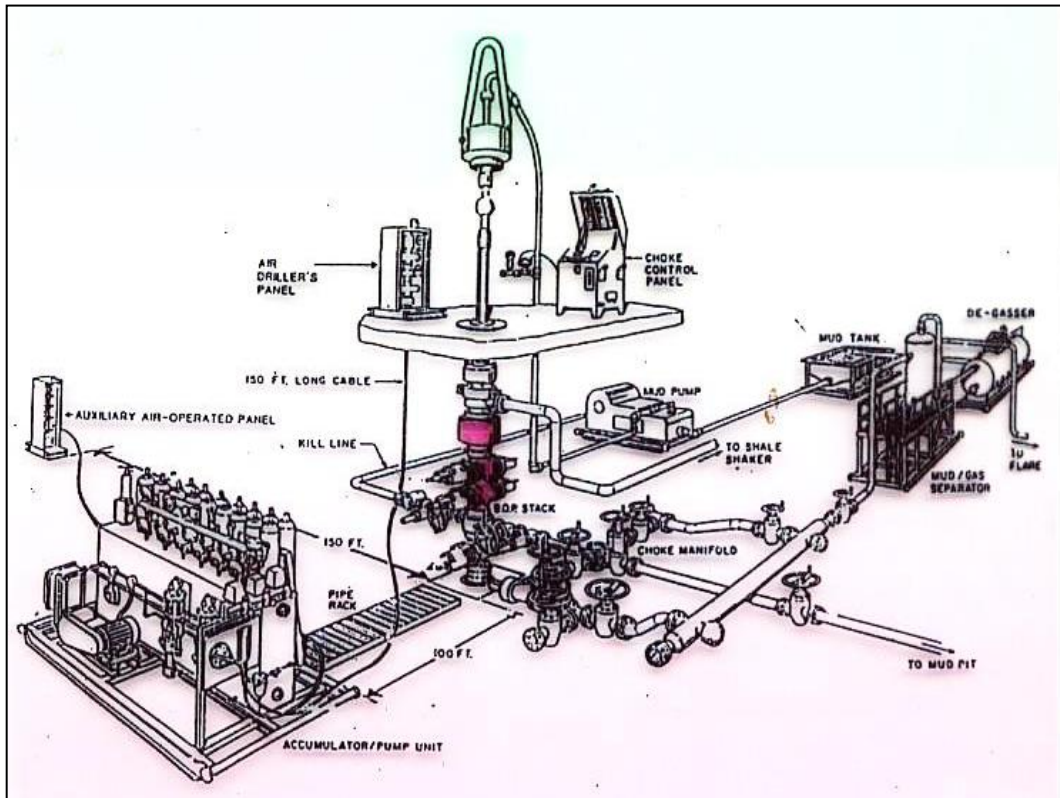
Gambar 4.37. BOP System
