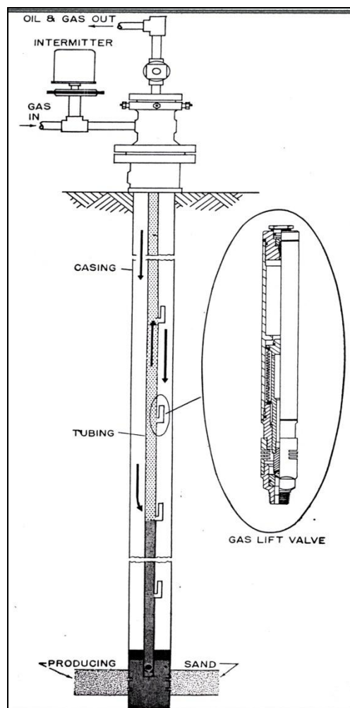
Gambar 8.5. Katup gas Lift
