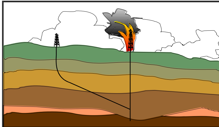
Gambar 3.10. Relief Well Drilling
