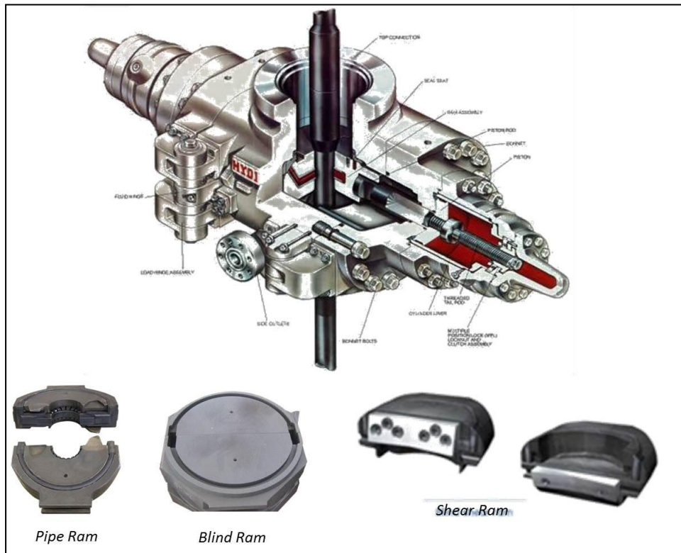
Gambar 4.41. Pipe Ram Preventer
