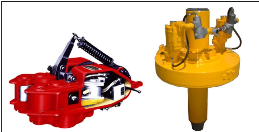
Gambar 4.22. Kelly Spinner
