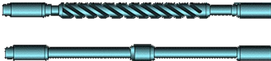
Gambar 4.27. Heavy Weight Drill Pipe
