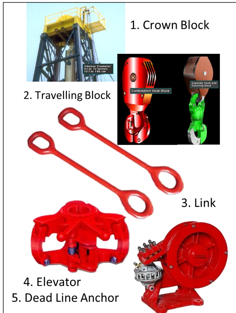
Gambar 4.8. Overhead Tools
