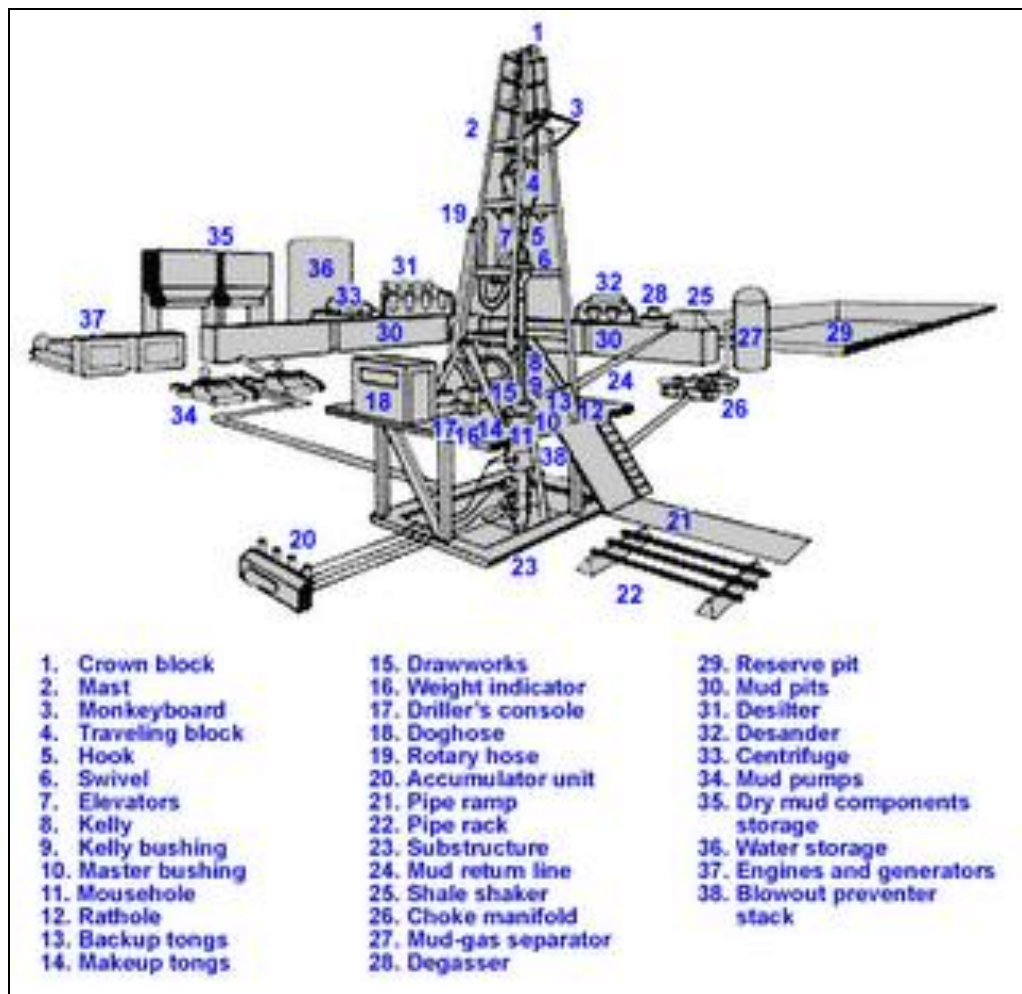
Gambar 4.1. Rig Equipment
