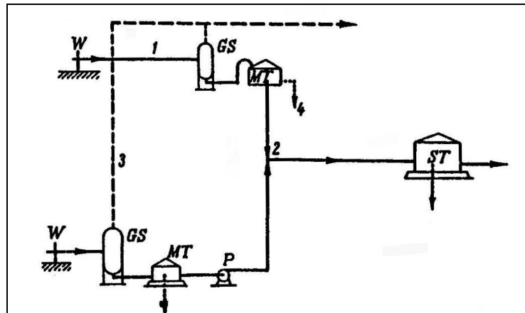
Gambar 8.12. Individual Oil and Gas Gathering System
