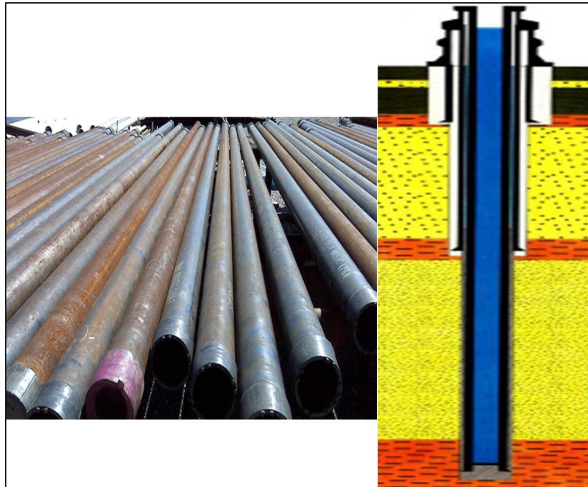
Gambar 5.4. Intermediate Casing
