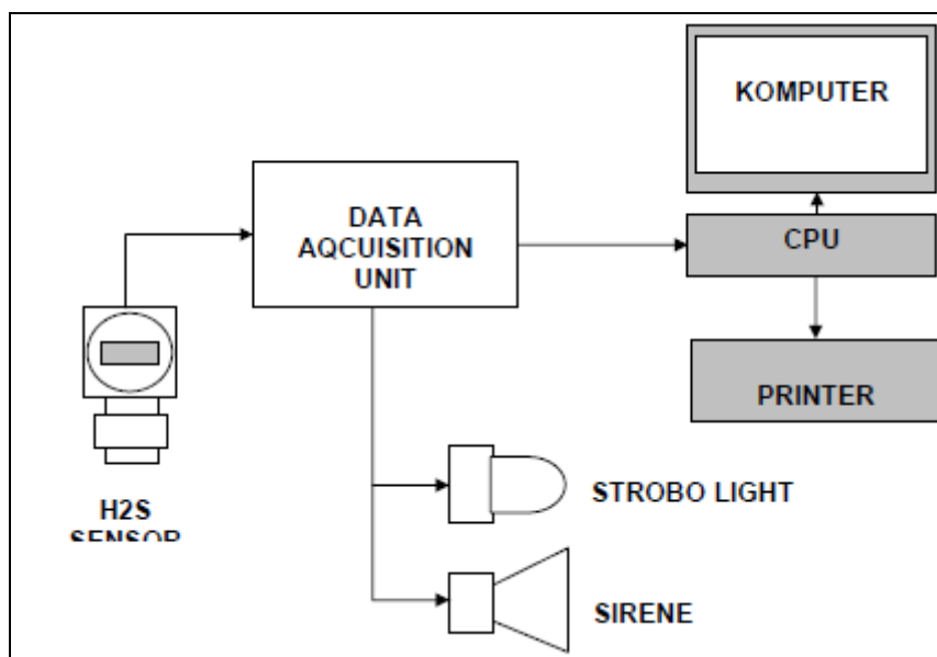
Gambar H 2 S Fixed Monitoring System
