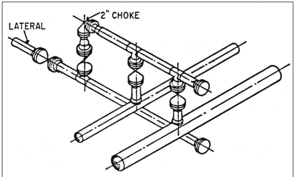
Gambar 8.14. Manifold
