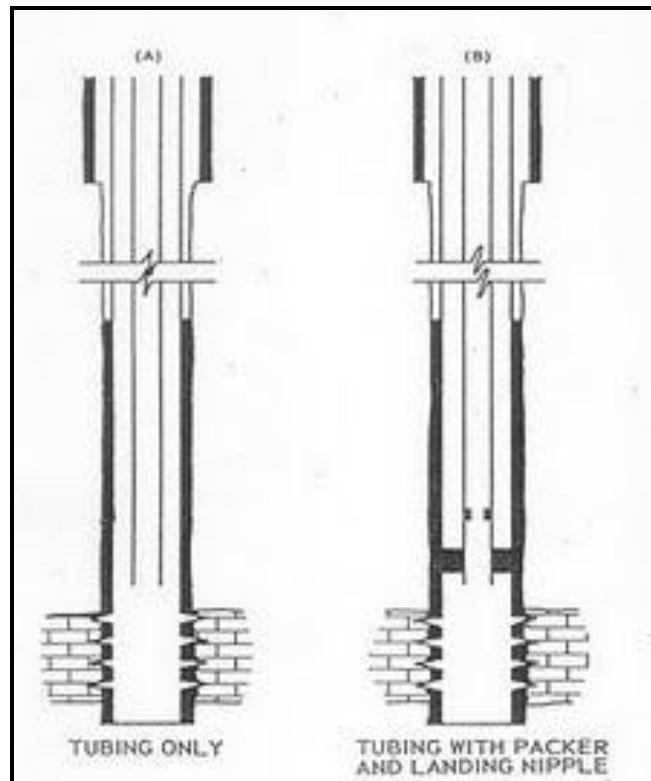
Gambar 6.2. Single Completion
