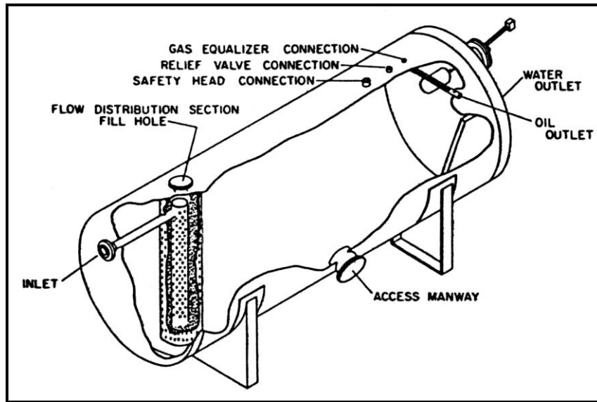
Gambar 8.22. Horizontal Oil Skimmer
