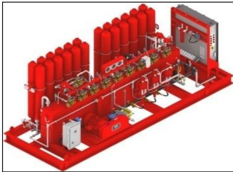
Gambar 4.43. Accumulator Unit
