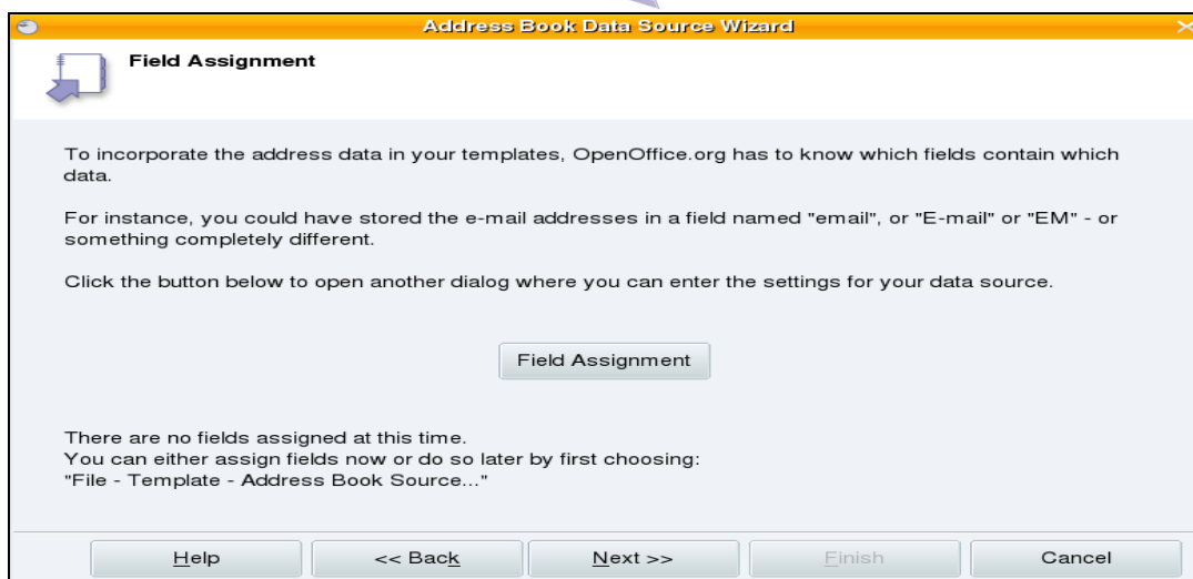
Gambar 5.25 Field Assignment
