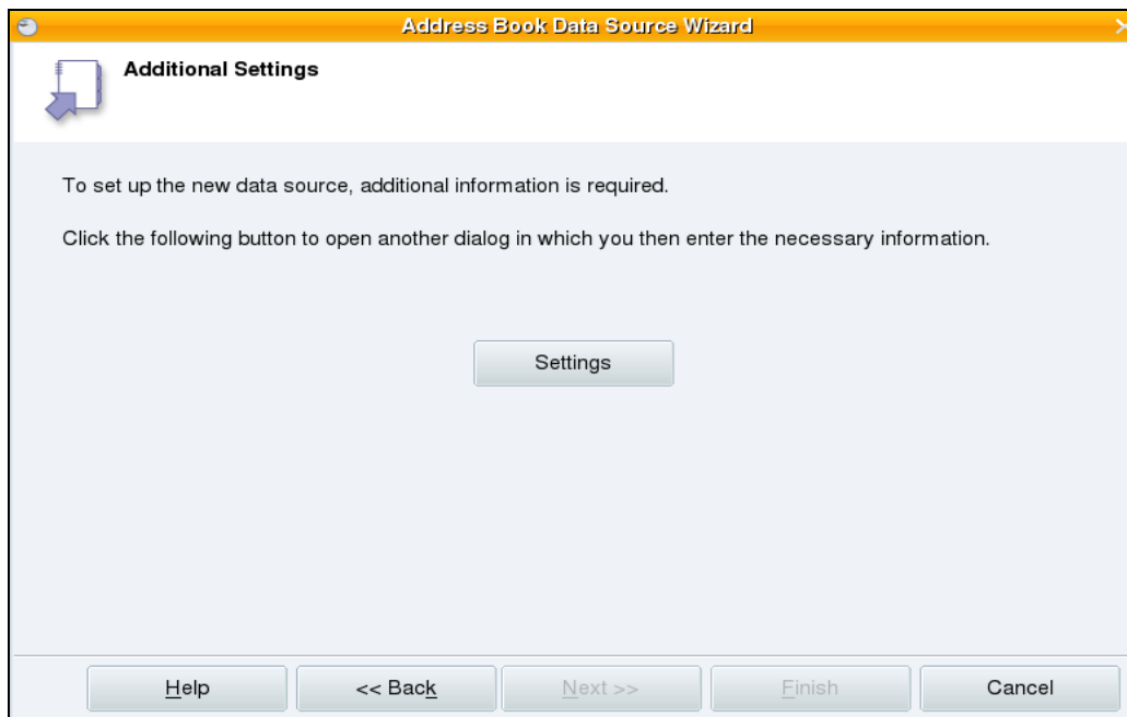
Gambar 5.21 Additional Settings
