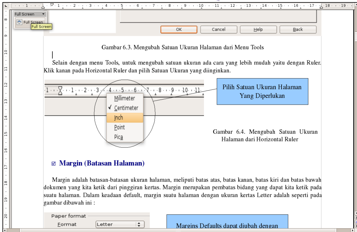
Gambar 6.8 Tampilan Fullscreen
