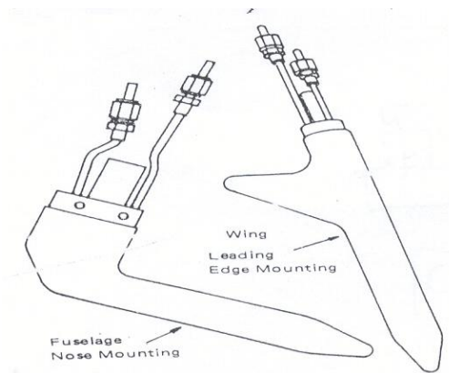
Gambar 1.8. Suction gage
