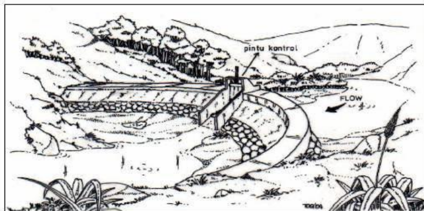
Gambar 32. Dam Pengendali (Tipe busur)
