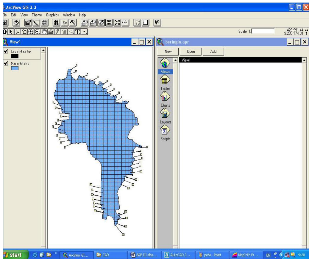
Gambar 10. Proses ArcView
