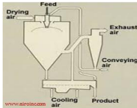
Gambar 37. Gambar pengering semprot ( Spray dryer )
