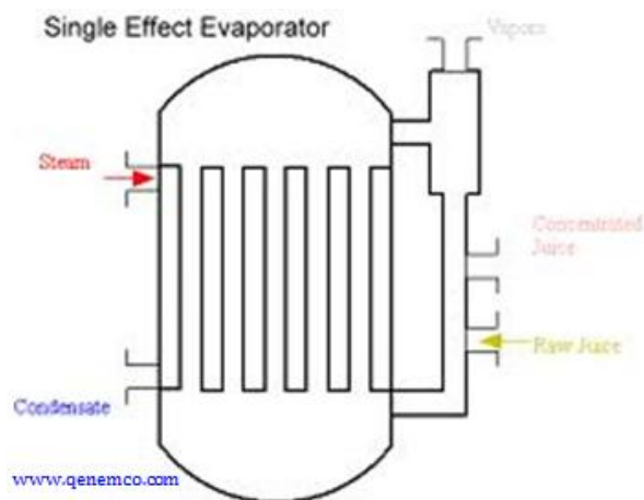
Gambar 42. Evaporator efek tunggal ( single effect evaporator )
