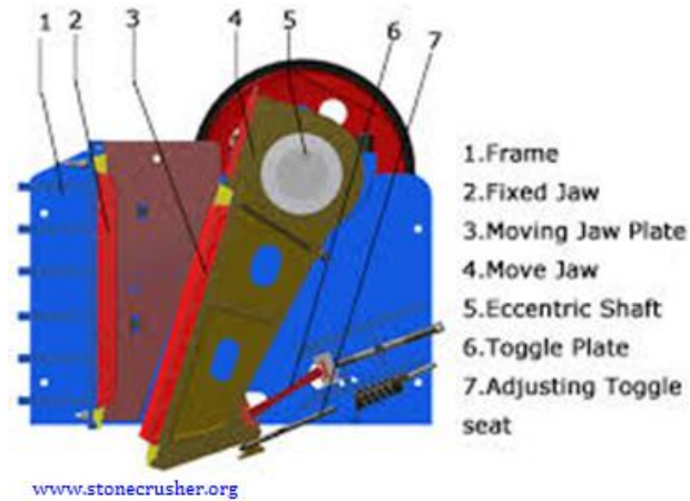
Gambar 14. Jaw crusher
