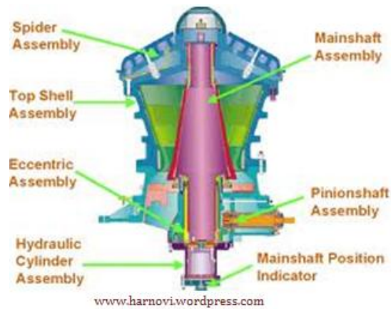
Gambar 15. Gyratory crusher .
