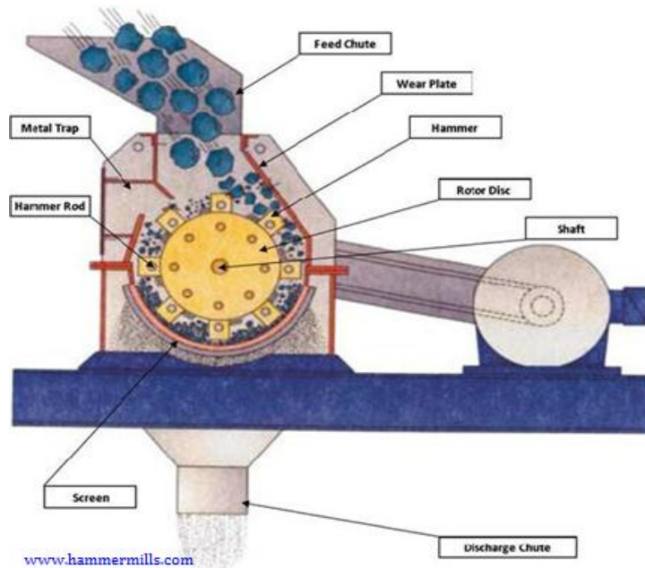
Gambar 10. Hammer Mill
