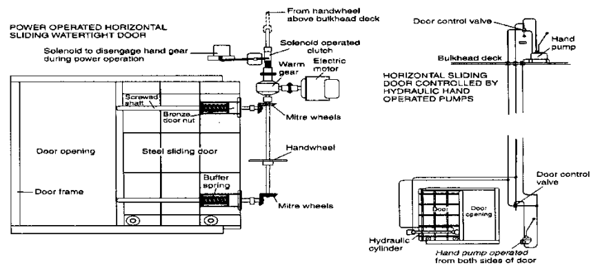
FIGURE 18.3 Watertight doors
