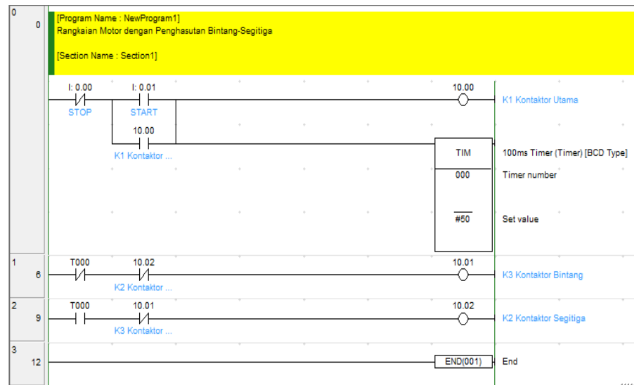
Gambar 99 Program Ladder Diagram PLC
