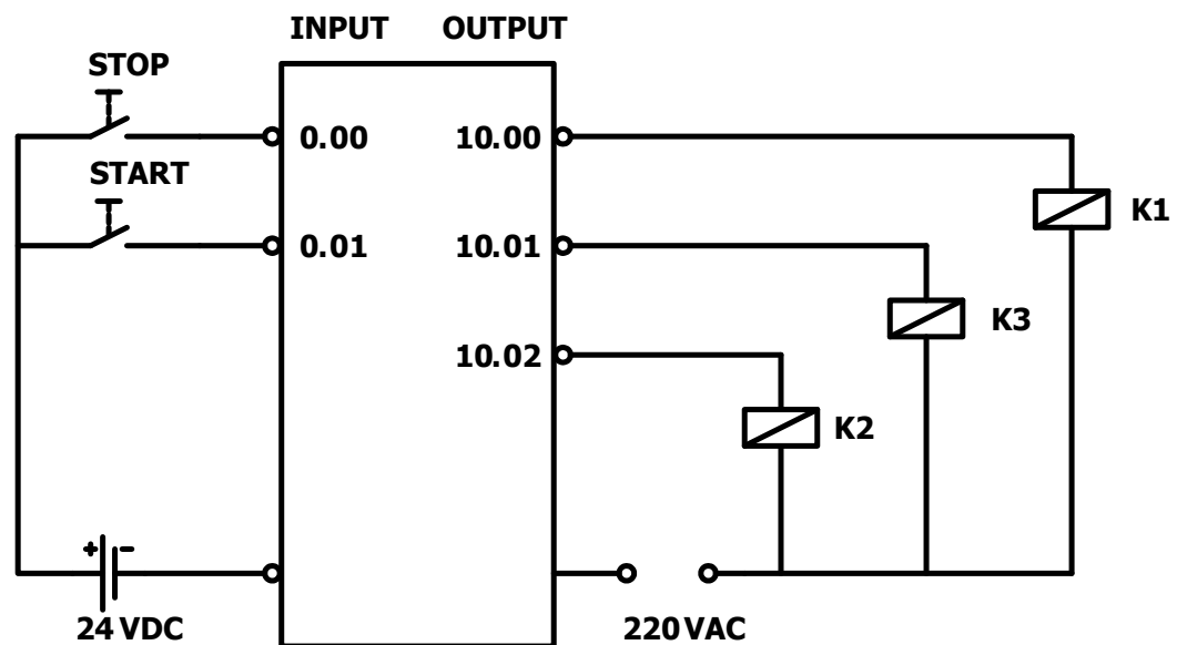
Gambar 98 Wiring PLC
