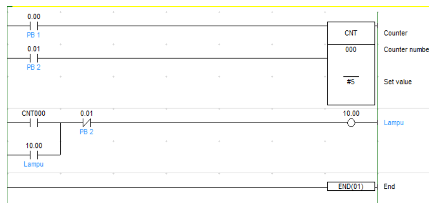
Gambar 33 Program Counter.
