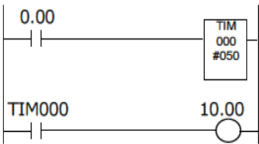
Gambar 30 Program tunda ON (1).
