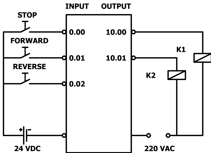
Gambar 92 Wiring PLC
