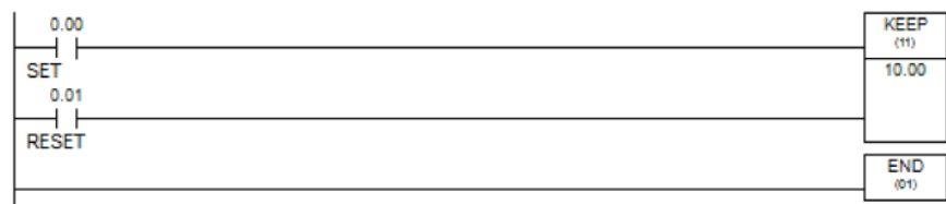
Gambar 34 Program KEEP.
