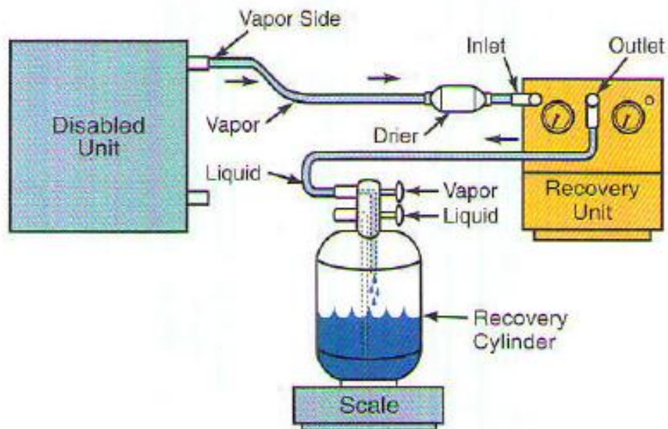
Gambar 5.10 Vapor Recovery Method
