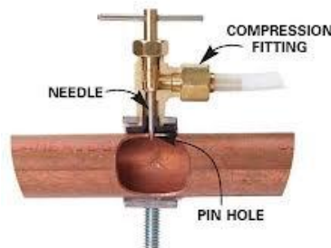
Gambar 2.4 tipikal Adjustable Line Tap Valve
