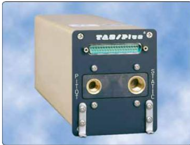
Teledyne's 90004 TAS/Plus air data computer (ADC) computes air data information from the pitot-static pneumatics system, aircraft temperature probe, and barometric correction device to help create a clear indication of flight conditions.
