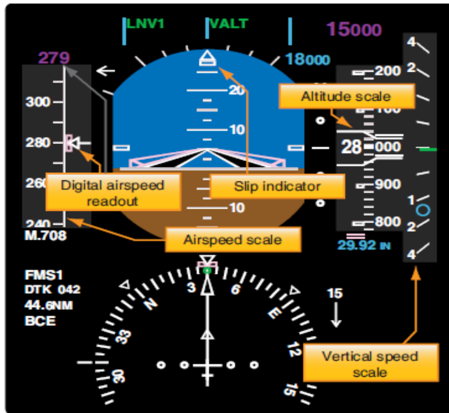
Gambar 1. An EFIS EADI displays an airspeed scale to the left of the horizon sphere and an altimeter and vertical speed scale to the right. The slip indicator is the small rectangle under the direction triangles at the top. This EFIS display presents all of the flight information in the conventional cockpit basic T.
