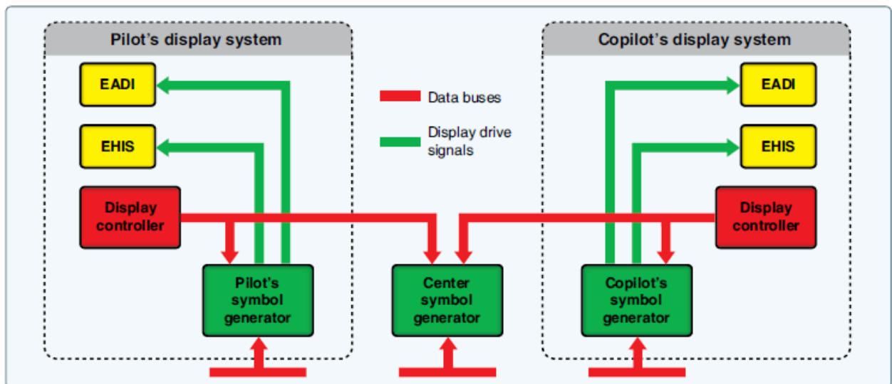
Gambar 2. A simplified diagram of an EFIS system. The EADI and EHIS displays are CRT units in earlier systems. Modern systems use digital displays, sometimes with only one multifunctional display unit replacing the two shown. Independent digital processors can also be located in a single unit to replace the three separate symbol generators
